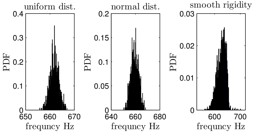
Figure 6: The PDF of 50th fundamental frequency for the uniform distribution (left), normal distribution (center) and smooth rigidity (right).
