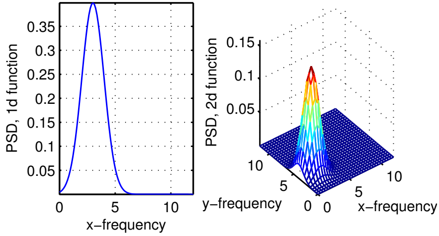
Figure 4. Examples of PSDs for the 1 and 2 dimensional random functions
