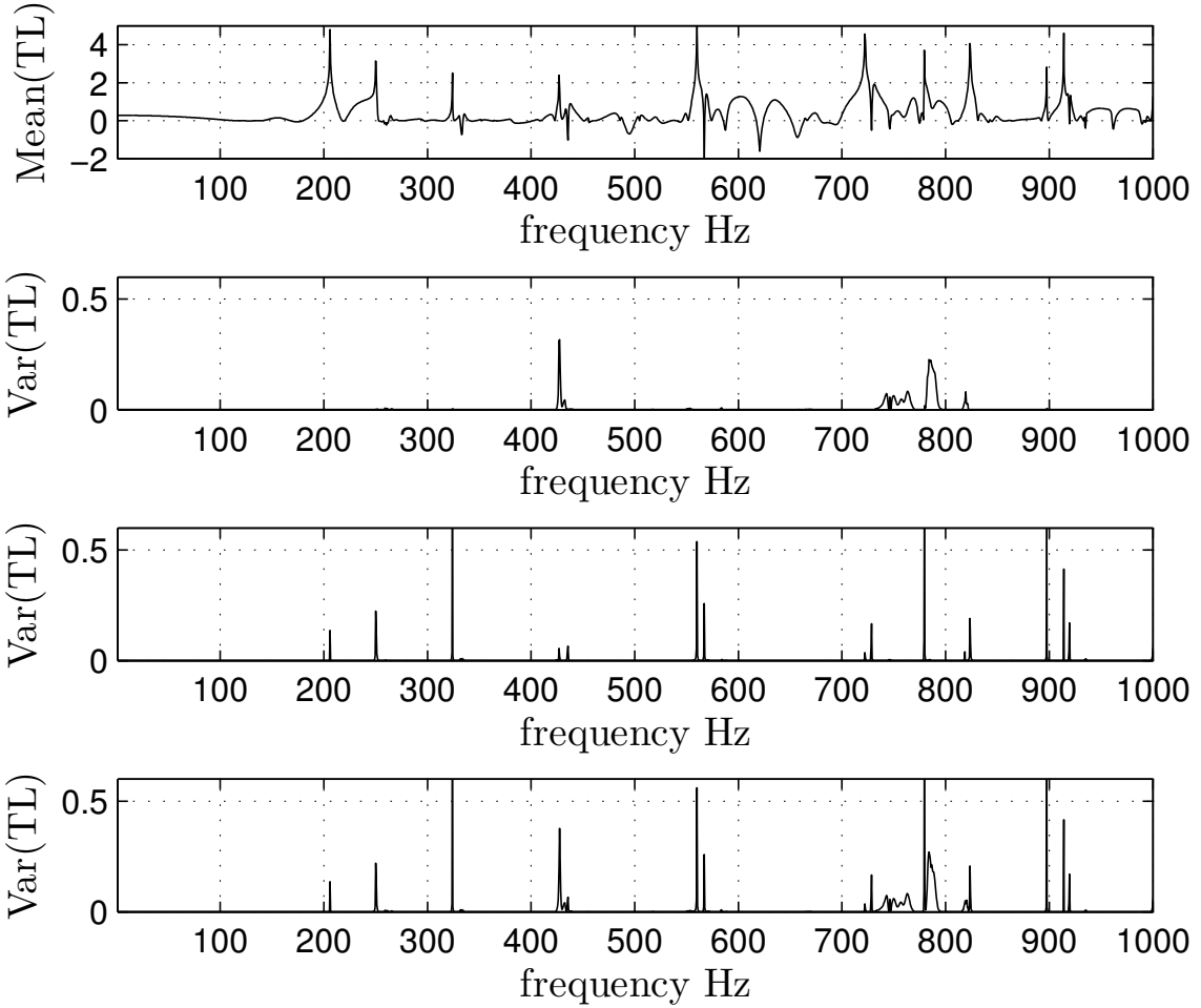
Figure 7: The mean of the TL (top). The variance of the TL when the slippage alone is randomized (top second), rigidity alone is randomized (top third) and both the slippage and the rigidities are randomized (bottom).
