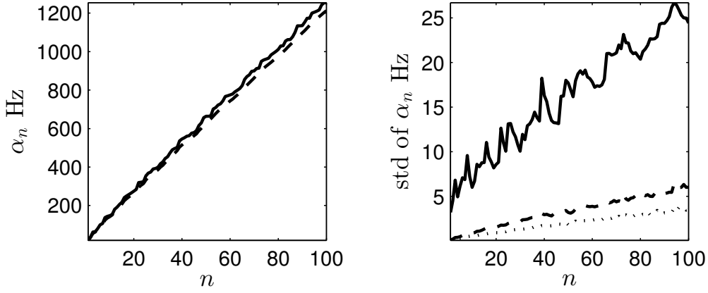
Figure 5: On the left, the mean of the fundamental frequencies for the discrete (solid) and the smooth (dashed) random rigidities. On the right, the standard deviation of the fundamental frequencies for uniformly distributed (dotted), normally distributed (dashed) and the smooth (solid) random rigidities. The standard deviation of all three cases is 10% of the average rigidity \bar{D} .
